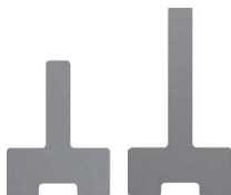
Chave falsa ×2 (47.5 mm, 67.5 mm)
